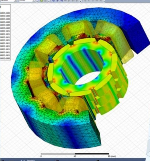
3D machine design
