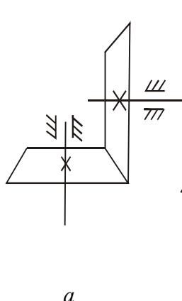
Fig. 8.10. Bevel gear: a – wheels in engagement; b – wheels on the kinematic diagram
