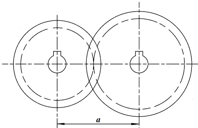
Fig. 8.3. Center distance
