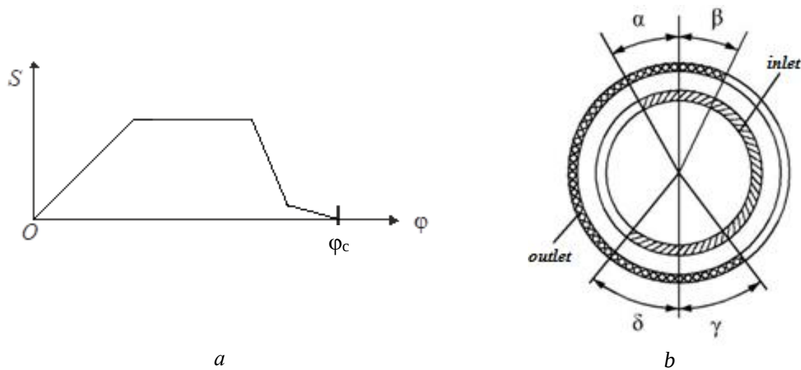
Fig. 1.1. Operational cyclogram of the machine:
